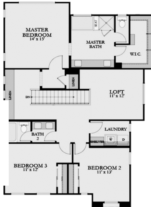
2ND FLOOR
